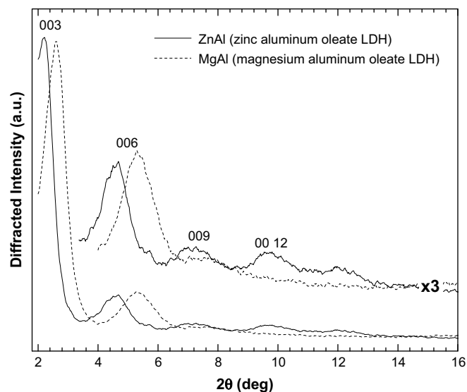
Fig. 2. X-ray diffraction traces of ZnAl and MgAl. The top traces are the same data at 3 × intensity to highlight the higher order Bragg reflections, where observable.
